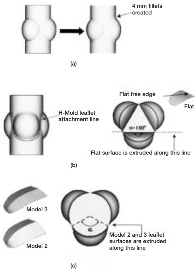
Figure 1: Modeling of aortic valve. a) Creation of sinus fillets; b) flat leaflet construction; c) model 2 and 3 leaflets.
