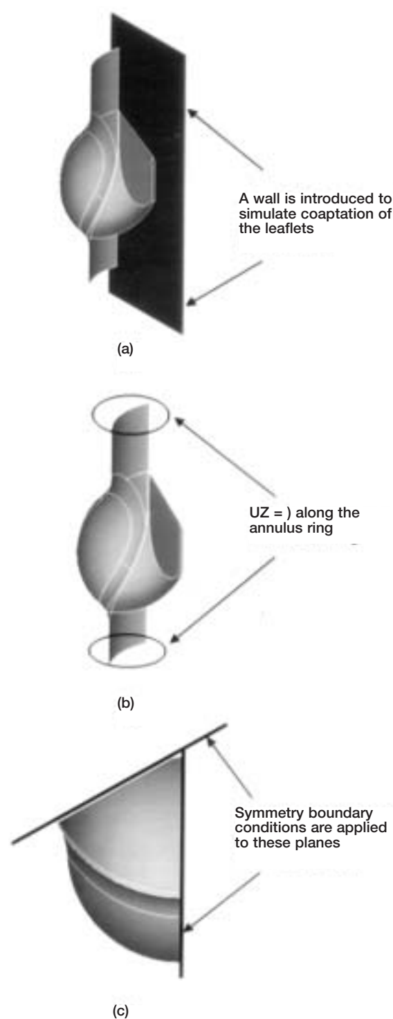
Figure 2: Application of boundary conditions. A) Introduction of wall to simulate contact between the leaflets. b) The annulus rings were constrained in the z direction. c) Symmetry boundary conditions applied to simulate full aortic root loading.
