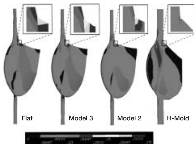
Figure 3: Contours of von Mises stress distribution on models with maximum stress insets. The color code bar shows the von Mises stress ranges of the models (in MPa).
